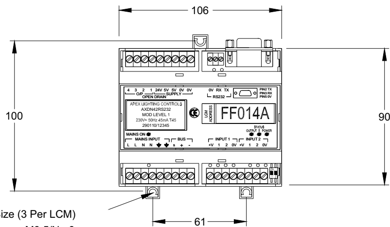
Panel Mounting
