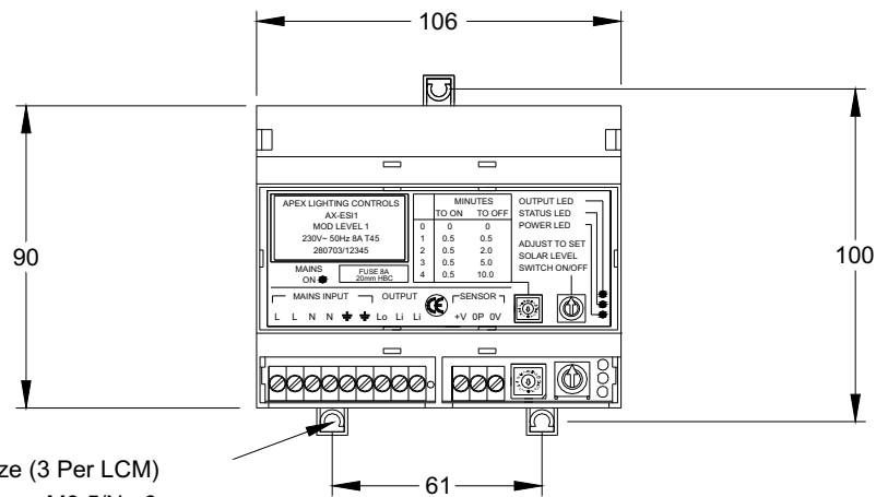
Panel Mounting
