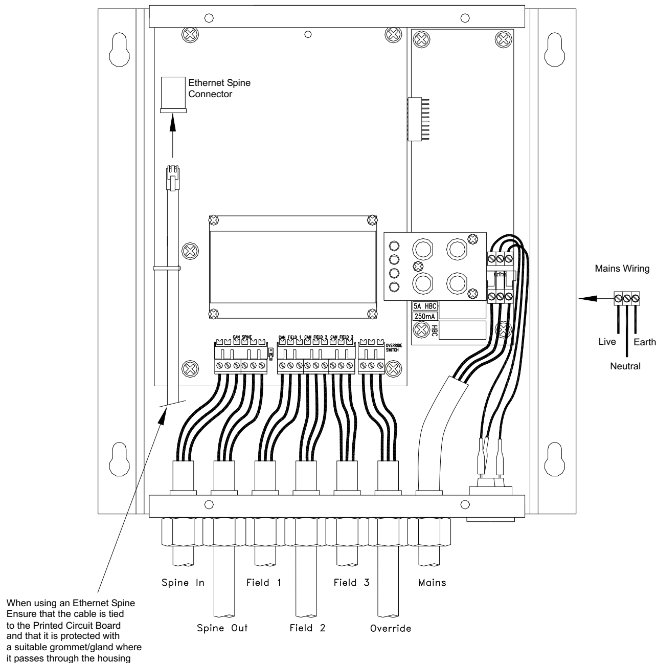
Spine/Field Bus Connector Wiring
