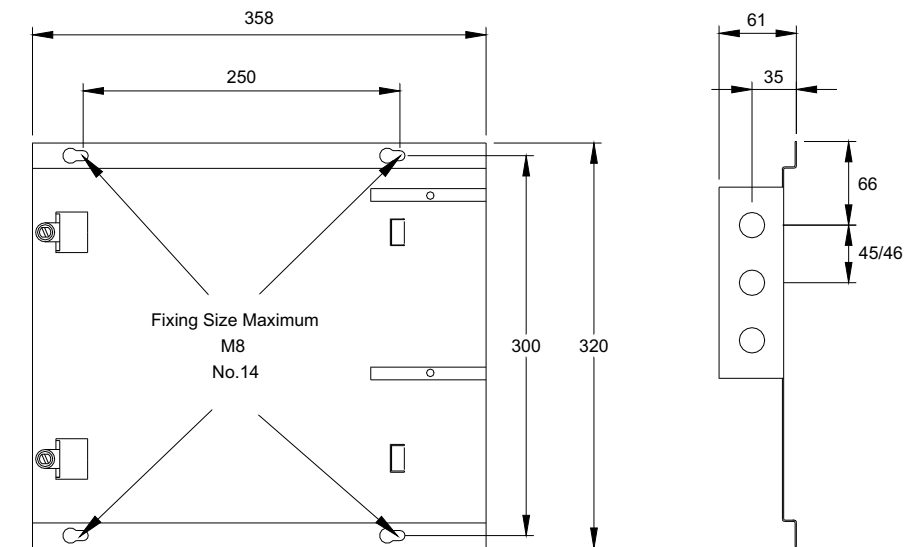
1/2 Turn Fixing
