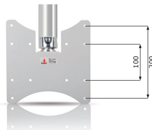
Standard VESA 100 and 200 mounting interface
